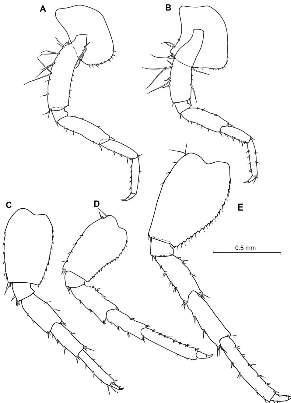
Fig. 4. Quadrivisio laleyi sp. nov. A–B., D–E. Holotype, ♂, 7.5 mm, MNHN IU-2017-209. C. Paratype, ♂, 7.6 mm, MNHN IU-2017-210. A. Pereopod 3. B. Pereopod 4. C. Pereopod 5. D. Pereopod 6. E. Pereopod 7.
